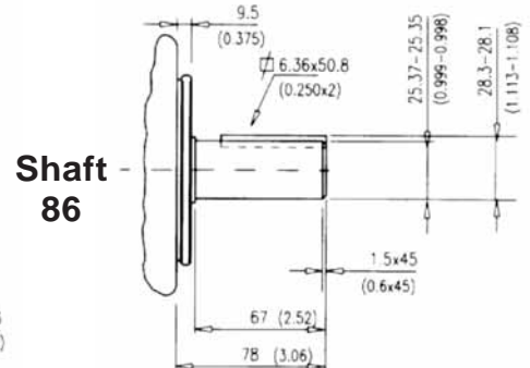
max torque capability: 400 Nm (3560 lb. in.)
