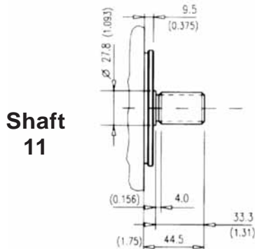
max. torque capability : 320Nm (2800 lb.in.)
